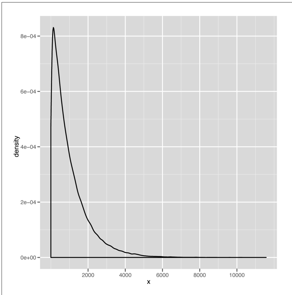
Figure 2-19. Skewed distribution
