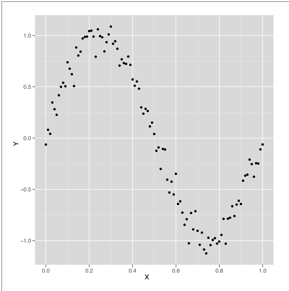
Figure 6-3. Nonlinear data
